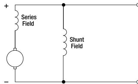
Figure 12-31. Compound motor.
