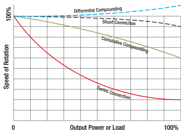
Figure 12-32. Load characteristics of DC motors.
