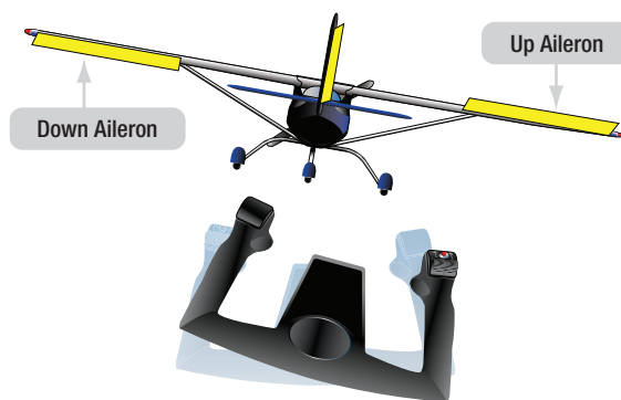
Figure 1-5. Differential aileron control movement. When one aileron is moved down, the aileron on the opposite wing is deflected upward.
