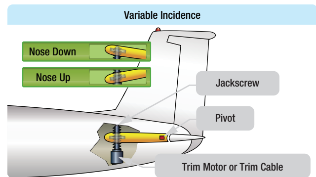
Figure 1-10. Some airplanes, including most jet transports, use an variable stabilizer to provide the required pitch trim forces.
