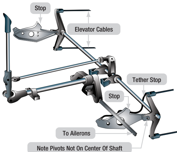
Figure 1-6. Transferring control surface inputs from the cockpit.
