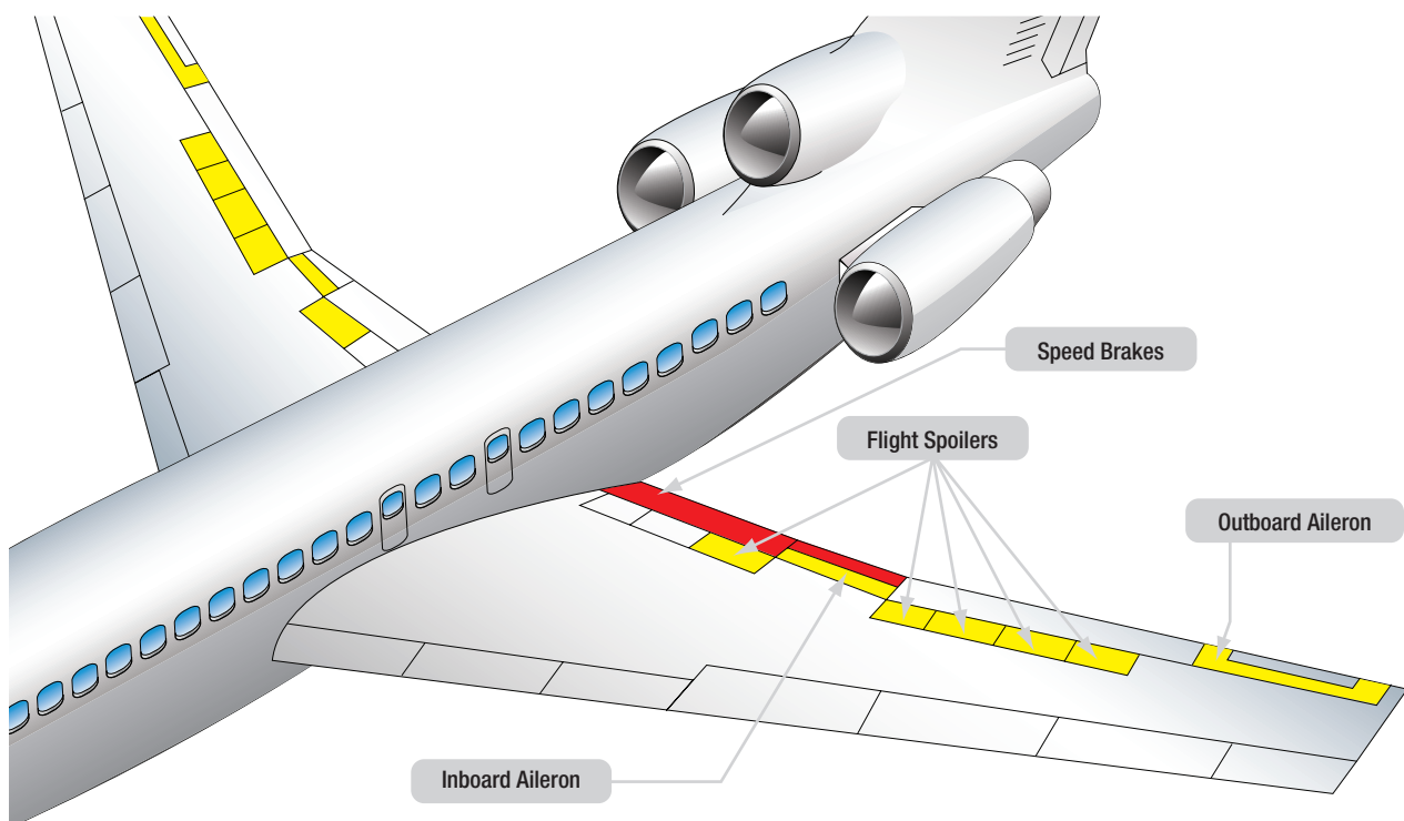
Figure 1-7. Typical flight control surfaces on a transport category aircraft.
