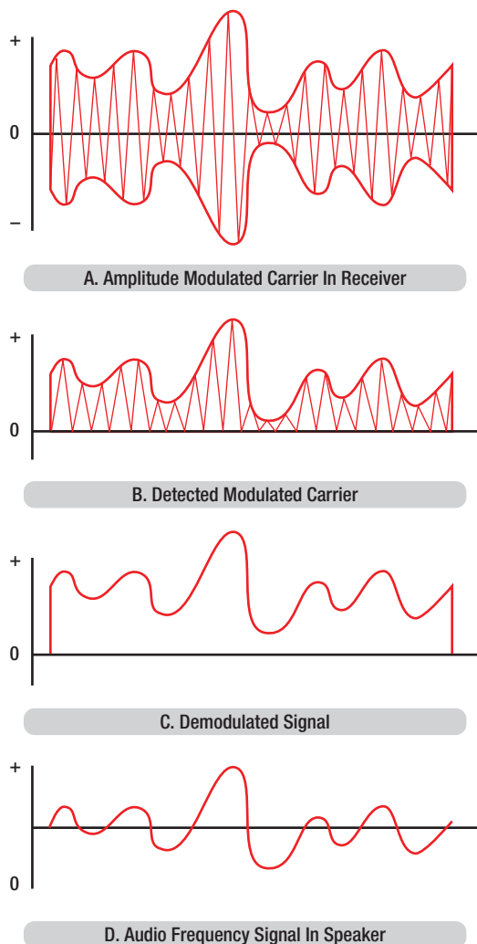
Figure 4-7. Demodulation of a received radio signal involves separating the carrier wave from the information signal.
