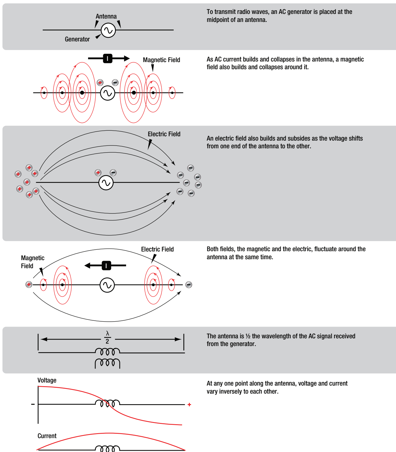
Figure 4-3. Radio waves are produced by applying an AC signal to an antenna. This creates a magnetic and electric field around the antenna. They build and collapse as the AC cycles. The speed at which the AC cycles does not allow the fields to completely collapse before the next fields build, collapsing fields are then forced out into space as radio waves.
