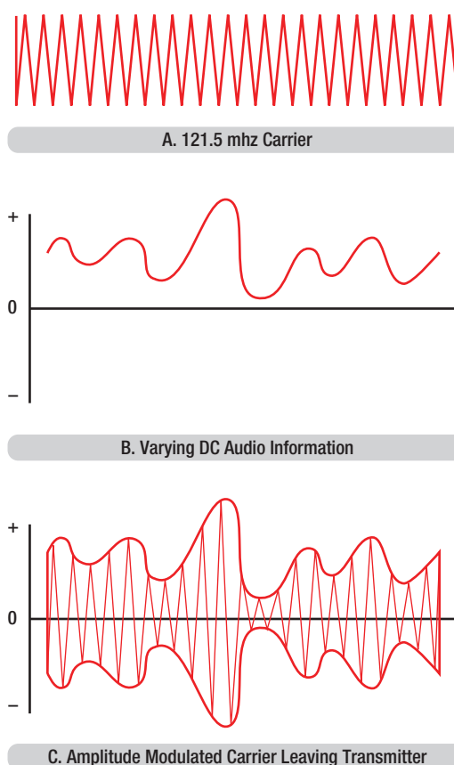
Figure 4-6. A DC audio signal modifies the 121.5 MHz carrier wave as shown in C. The amplitude of the carrier wave (A) is changed in relation to modifier (B). This is known as amplitude modulation (AM).
