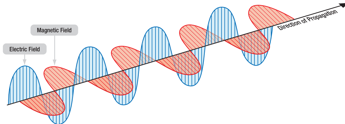
Figure 4-4. The electric field and the magnetic field of a radio wave are perpendicular to each other and to the direction of propagation of the wave.
