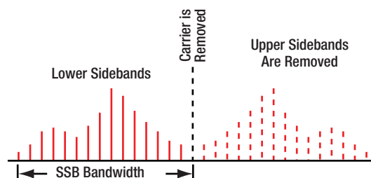
Figure 4-10. The additional frequencies above and below the carrier wave produced during modulation with the information signal are known as sidebands. Each sideband contains the unique information of the information signal and can be transmitted independent of the carrier wave and the other sideband.
