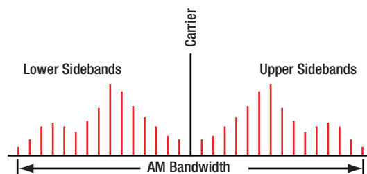
Figure 4-9. The bandwidth of an AM signal contains the carrier wave, the carrier wave plus the information signal frequencies, and the carrier wave minus the information signal frequencies.
