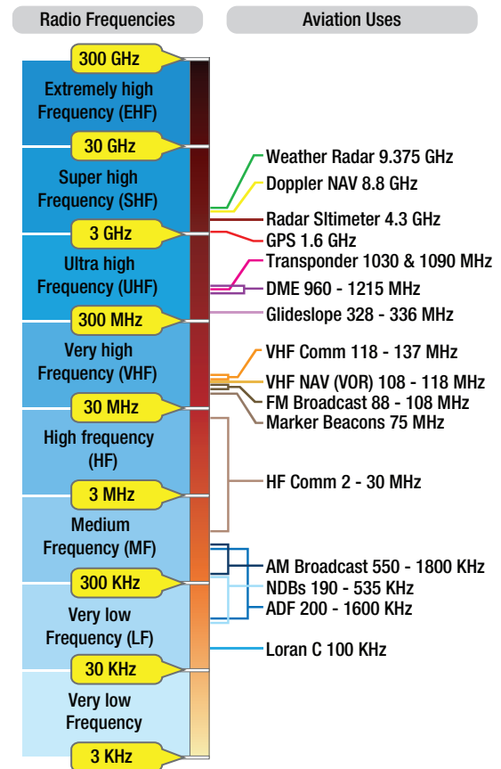
Figure 4-2. There is a wide range of radio frequencies. Aviation does not use very low frequencies or extremely high frequencies.
