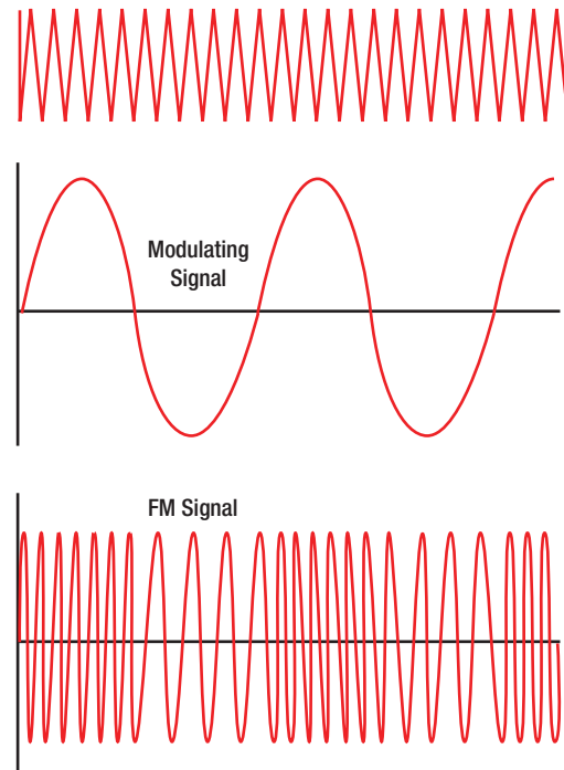
Figure 4-8. A frequency modulated (FM) carrier wave retains the consistent amplitude of the AC sign wave. It encodes the unique information signal with slight variations to the frequency of the carrier wave. These variations are shown as space variations between the peaks and valleys of the wave on an oscilloscope.
