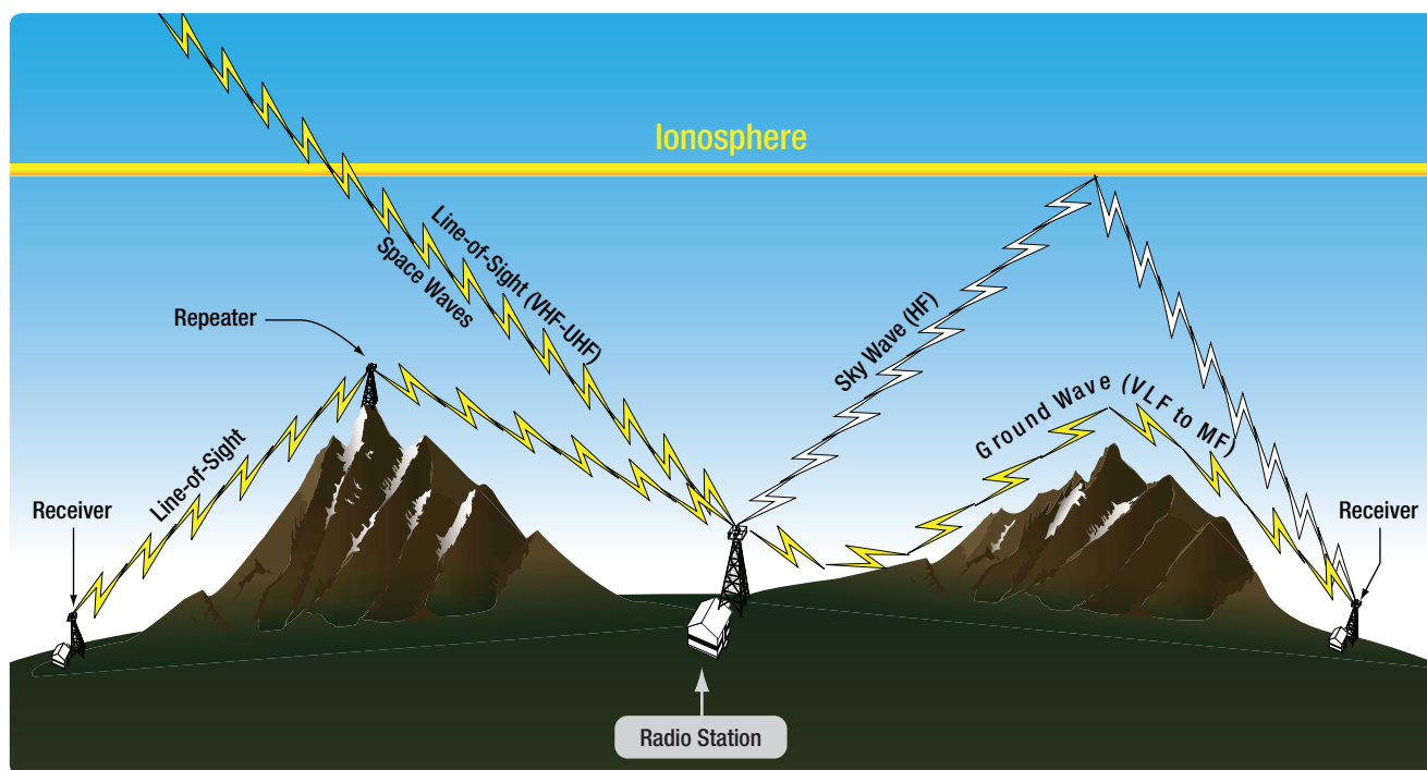
Figure 4-5. Radio waves behave differently in the atmosphere depending in their frequency.
